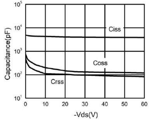
Figure 9. Capacitance
