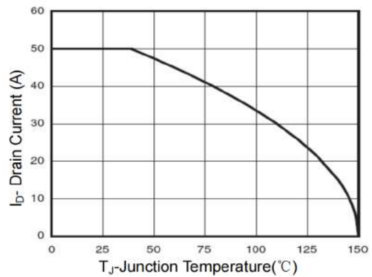
Figure 5. Drain Current
