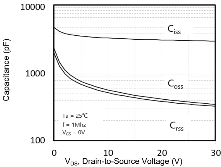
Figure 7 . Capacitance Characteristics
