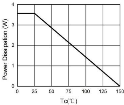
Figure 3. Power Dissipation
